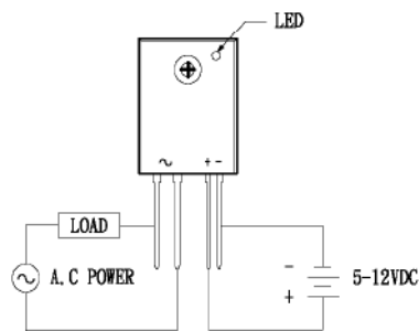
Fig.8 WIRING DIAGRAM
