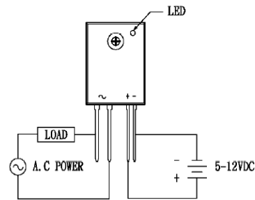
Fig.8 WIRING DIAGRAM
